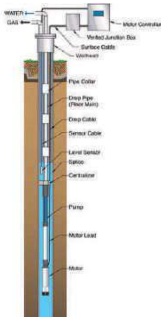
Technical Layout of Submersible Pump
